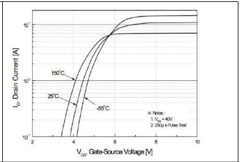
FIG.2-TRANSFER CHARACTERISTICS
