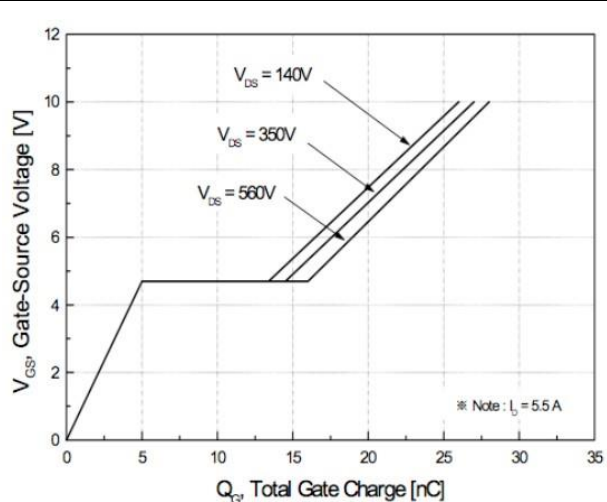
FIG.6-GATE CHARGE CHARACTERISTICS
