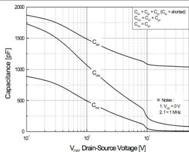
FIG.5-CAPACITANCE CHARACTERISTICS
