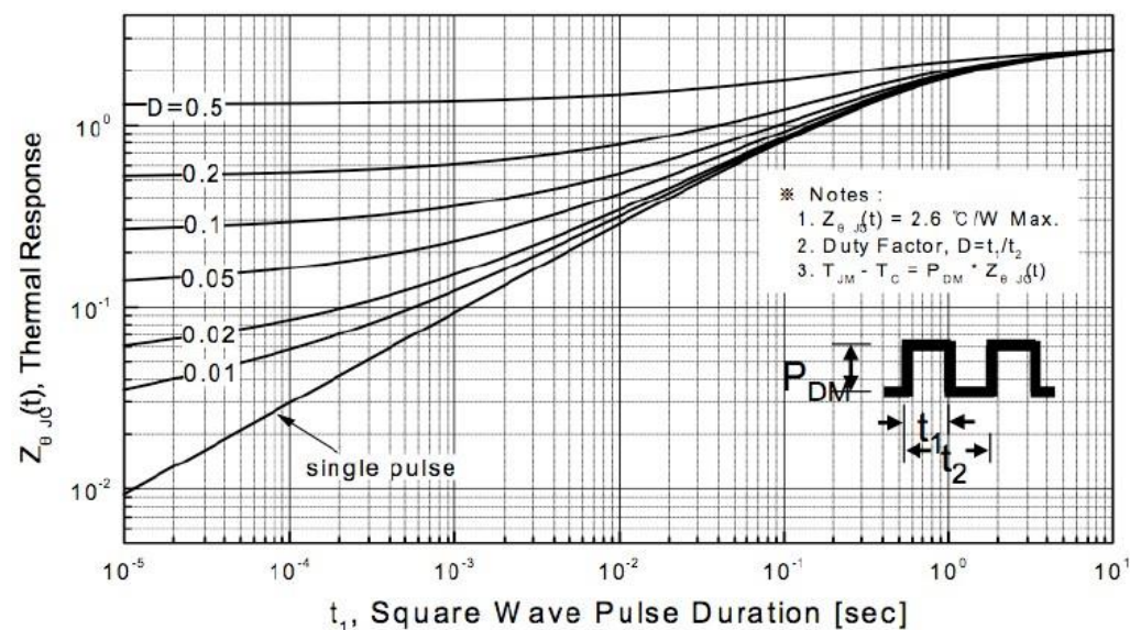
FIG.11-TRANSIENT THERMAL RESPONSE CURVE
