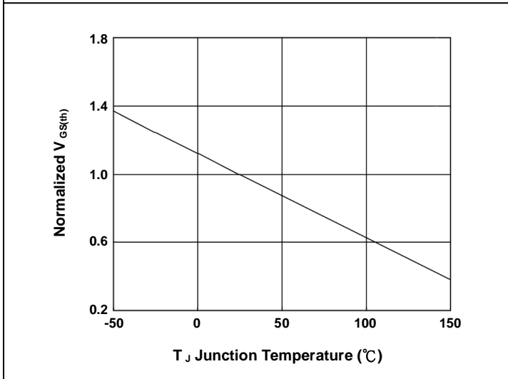
FIG.3-Normalized V_{GS(th)} vs. T_J
