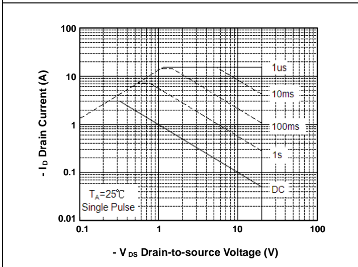
FIG.5-Safe Operating Area
