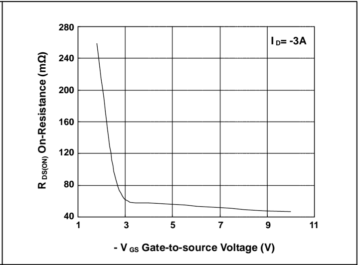
FIG.2-On-Resistance vs. G-S Voltage
