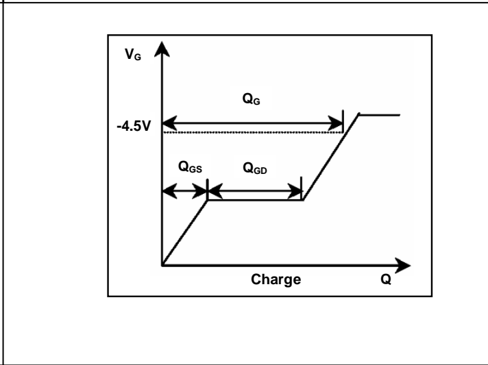
FIG.10-Gate Charge Waveform
