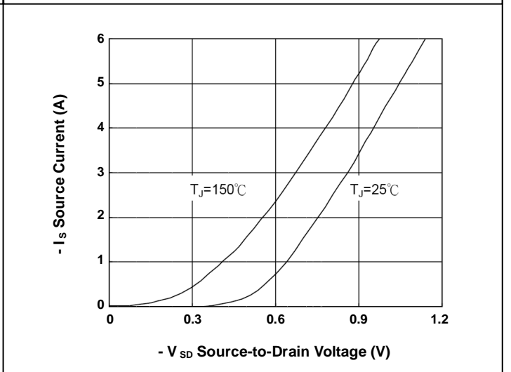
FIG.6-Forward Characteristics of Reverse
