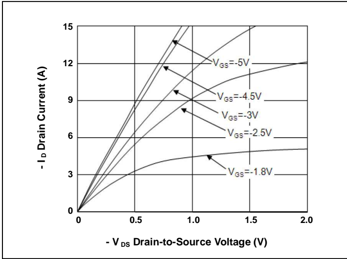
FIG.1-Typical Output Characteristics
