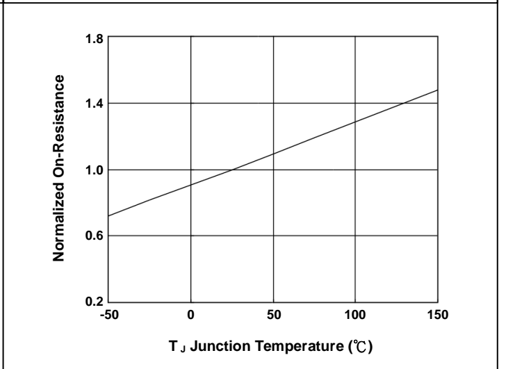
FIG.4-Normalized R_{DS(on)} vs. T_J
