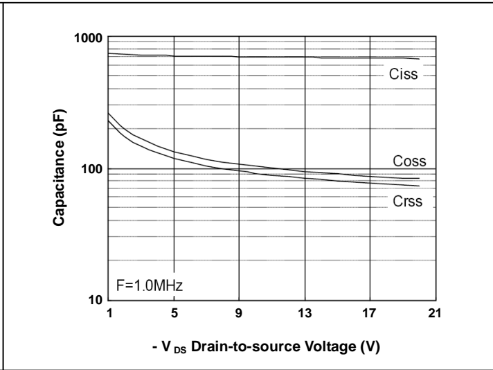
FIG.8-Capacitance Characteristics
