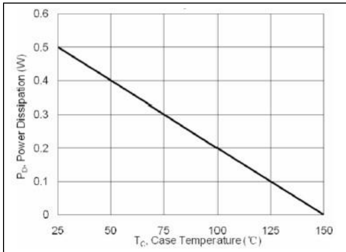
FIG.1 – MAXIMUM POWER DISSIPATION VS CASE TEMPERATURE
