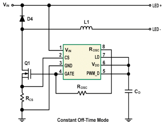
Figure 4. Constant Off-Time Mode
