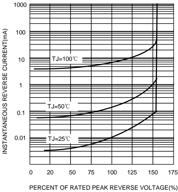
FIG.5-TYPICAL JUNCTION
